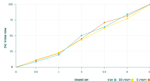
Vitamin C + Vitamin D + Zinc Beadlets - Release Profile
